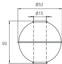
F01 Floater Ø 50x50 mm Stainless steel (MST/MSP/MSTL)
