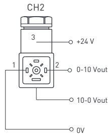
0-10V and 10-0V Output
