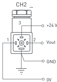
0-10V or 10-0V Output
