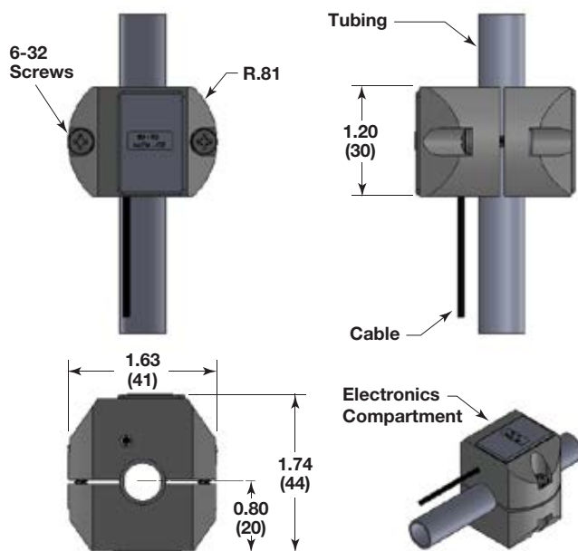
BDRI Sensor Dimensions inches (mm)
