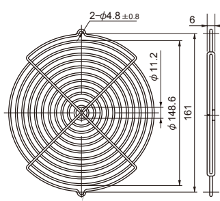
GUARD 172
